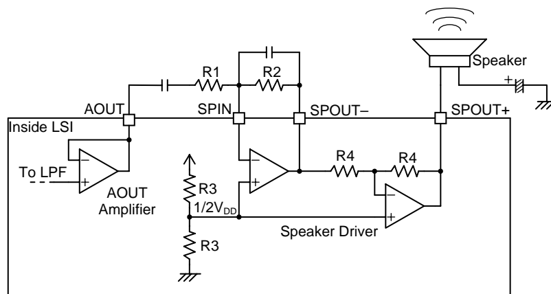
Figure 25 Speaker Connection
